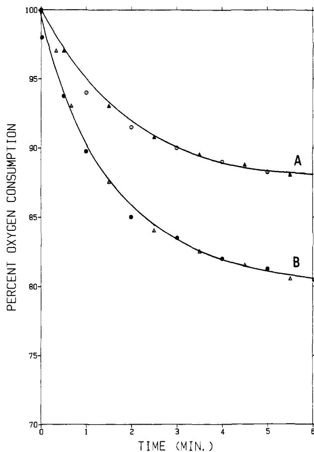
Figure 4. Time course of oxygen uptake and inactivation rate in the absence and presence of DBM/PEDA preformed products. The reaction mixture contained 10 mM fumarate, 0.25 mg/mL of catalase, 0.5 \mu M \text{CuSO}_4 , 20 mM ascorbate, and 20 mM PEDA in 0.125 M NaOAc, pH 5.0 (2.575 mL is the total volume). The reaction, run at 37 ^\circ\text{C} , was initiated by adding 4.4 \mu\text{g} of DBM and was monitored by the standard dissolved oxygen electrode assay (curve A, ○). After total inactivation of the enzyme, the system was resaturated with air, an identical aliquot of DBM was added, and the reaction monitored (curve A, ▲). After total inactivation a third aliquot of DBM containing twice as much enzyme (8.8 \mu\text{g} ) was added, and reaction was monitored (curve B, △). After total inactivation of the enzyme, the system was resaturated with air, and another identical aliquot (8.8 \mu\text{g} ) of DBM was added (curve B, ●).
