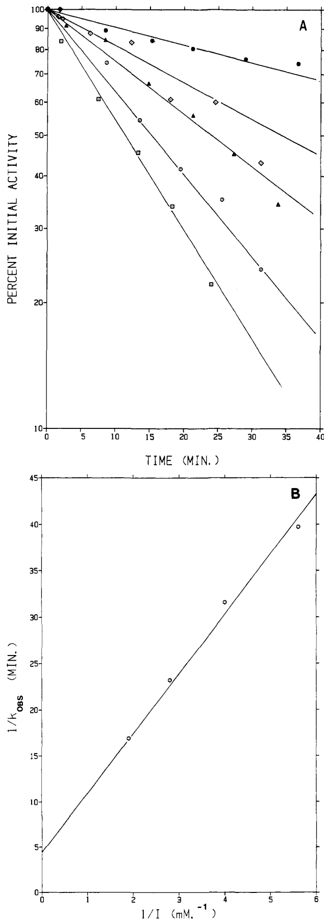
Figure 3. Kinetics of time dependent inactivation of DBM with PEDA. Panel 3A: (□) 0.537 mM; (○) 0.357 mM; (△) 0.250 mM; (◇) 0.179 mM; (●) 0.537 mM PEDA + 20 mM tyramine (conditions as described in the Materials and Methods Section). Panel 3B: double reciprocal-plot of data from Figure 3A.
